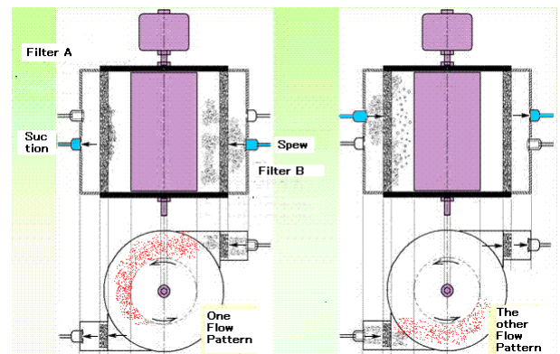
Fig.18. The double circulation system
