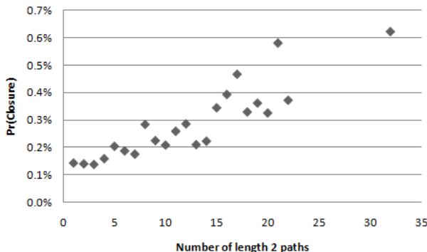
Figure 1: The number of closures between two authors increases with the number of length 2 paths.
