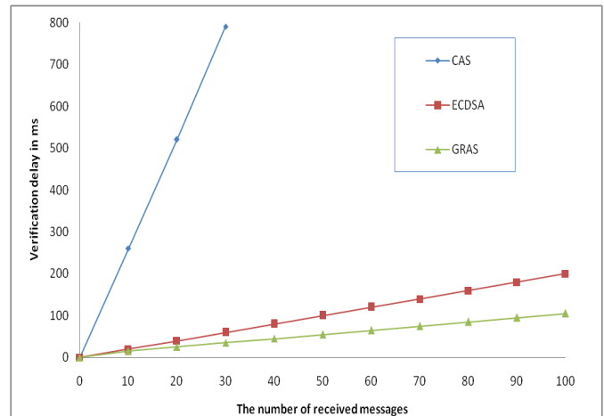
Figure 2: Verification delay for CAS, ECDSA and GRAS schemes
