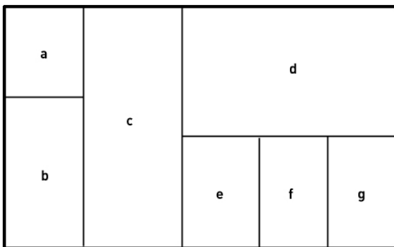
Figure 2: Treemap division
