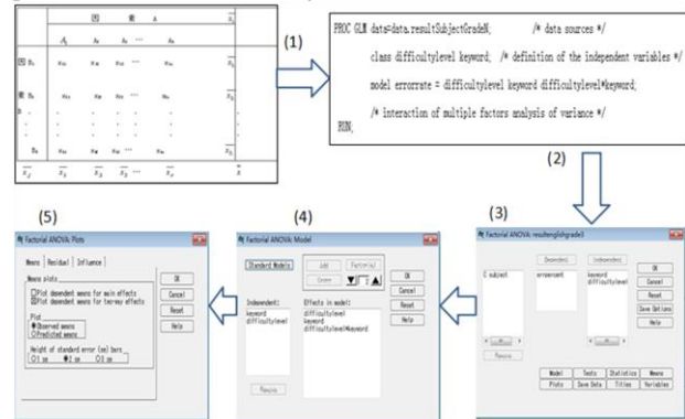
Fig. 4-3 ANOVA Data Result Process
