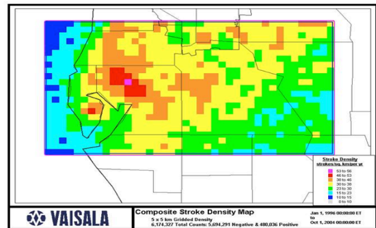
Fig. 7. Composite Lightning Strikes from Jan. 1996 to Oct 2004. The majority of strikes North-northeast of Tampa Bay Geospatially Correlate to the Eye Passage of Hurricanes Frances and Jeanne [7].
