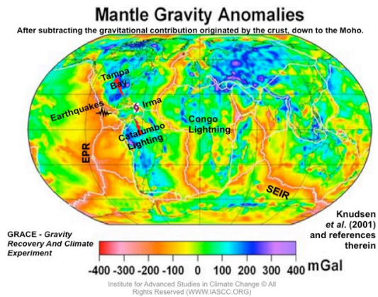
Fig. 3. Mantle gravity anomalies from GRACE satellite mission data [8] indicate EPR polar and continental circuit connections to Catatumbo, Tampa Bay lightning anomalies, and SEIR connections to the African Rift/Congo global lighting anomalies in Fig. 2.
