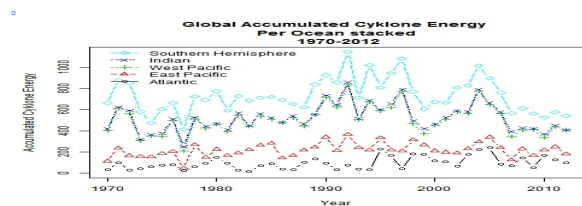
Fig. 11. This graph shows the development of Accumulated Cyclone Energy (ACE) by ocean basins. The figures are stacked on top of each other for each basin [25].
