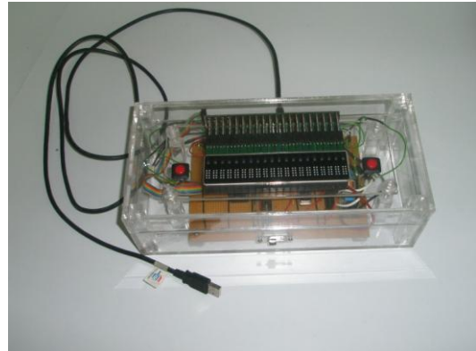
Figure 3: Refreshable Braille Display
