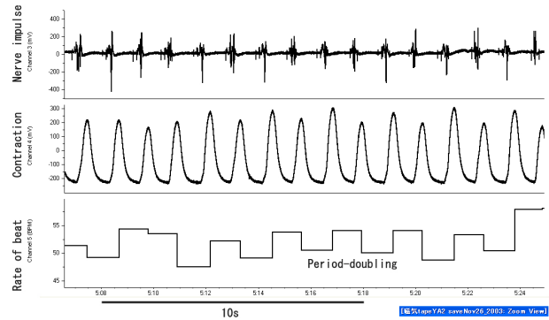
Figure 2. Alternative beats. The same heart in Figure 1.
