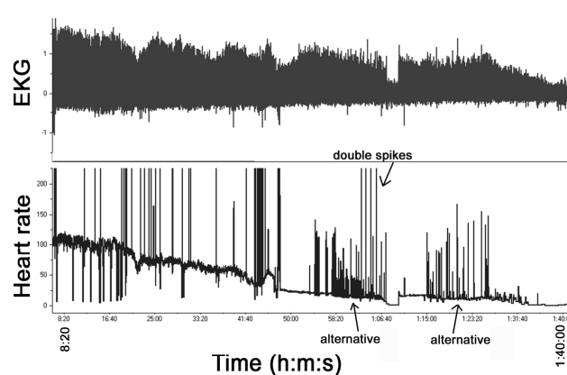
Figure 8. One and a half hour long EKG was taken at the last moment of the crayfish's life. Alternans occurred when this wild crayfish died.
