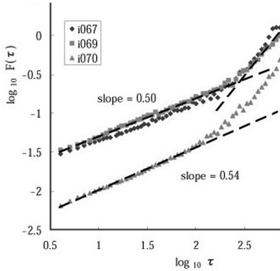
Figure 4. DFA of Alternans. Three examples of isolated hearts of Japanese spiny lobsters. All slop exhibited ~0.5.
