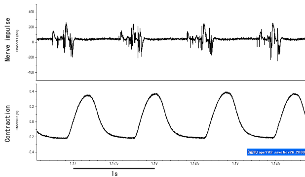
Figure 1. Pacemaker discharge and force of contraction recorded from dissected heart of hermit crab.
