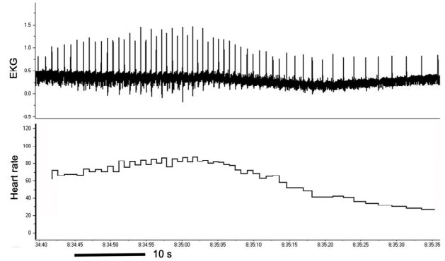
Figure 6. Alternans occurs at the top speed. Freely moving mutant (white) crayfish. The same crayfish in Figure 5.
