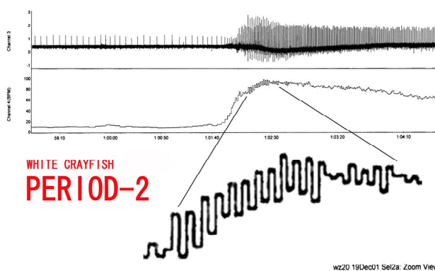
Figure 5. Spontaneously occurred alternans in freely moving mutant (white) crayfish.
