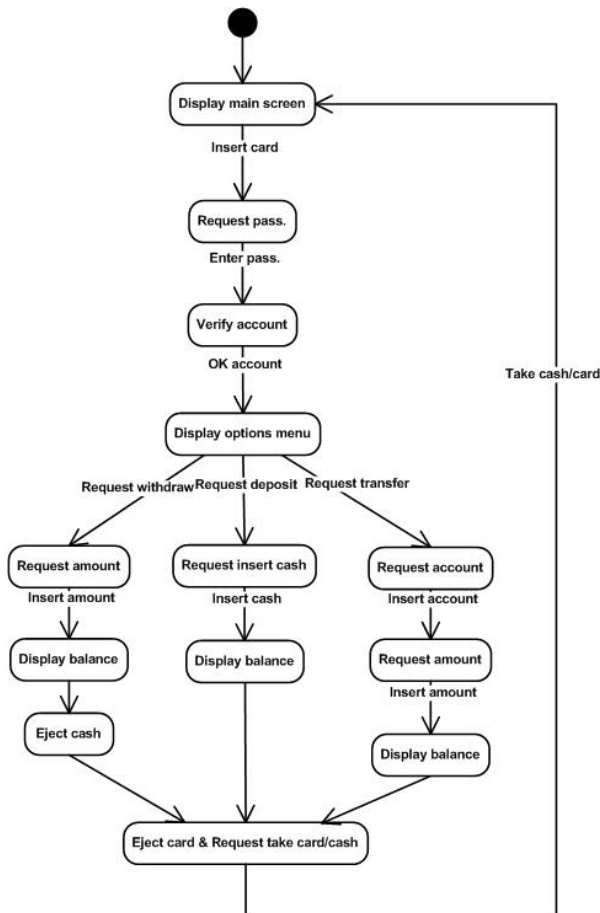
Fig.9. Refined state machine diagram for object ATM
