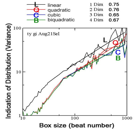
Figure 3. An example DFA computation. The DFA at a final step needs to calculate the slope in the graph of Box-size vs. Variance. But in the mid-way of the DFA, the least-mean square methods were involved, with linear-, quadratic-, cubic-, and bi-quadratic-fitting methods (details are not shown here). This graph is the final step. This was made after a measurement of such a least-mean square fitting function under a various Box size. Those measurements were done from the interval time series data, which was converted from the original EKG data. When linear-, quadratic-, cubic-, and bi-quadratic fitting were performed, finally we obtain a steady result of DFA calculation (for example, there is no big difference between C and B in the figure) the result of B was determined as the scaling exponent. This means, an approximate scaling exponent was determined, and is way down below from the normal value (i.e., 1.0) in this figure. The scaling exponent for this heart was about 0.7. Female 58.
