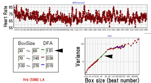
Figure 6. A DFA example for a person who has a high scaling exponent. Male 59.
