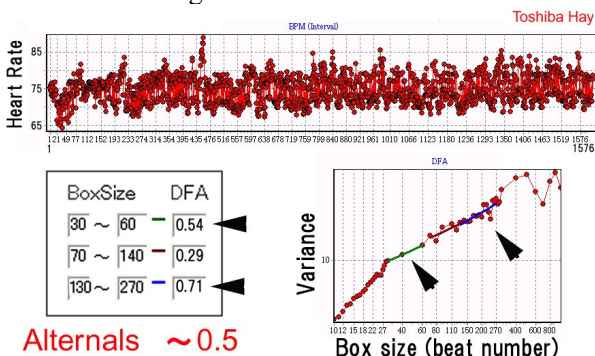
Figure 5. Alternans shows very low scaling exponents. Heart rate trace clearly shows an abnormality of its rhythm. The scaling exponents were 0.5 to 0.7 at different Box size. Male 55.
