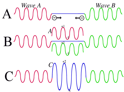
Figure 1 Constructive Interference
