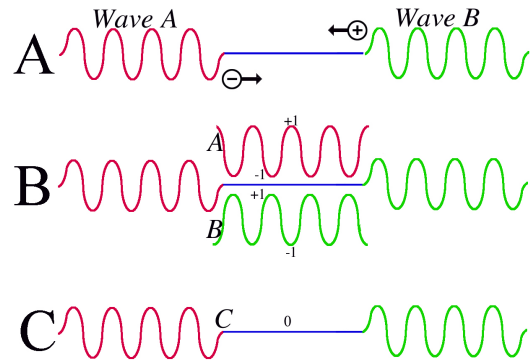
Figure 2 Destructive Interference
